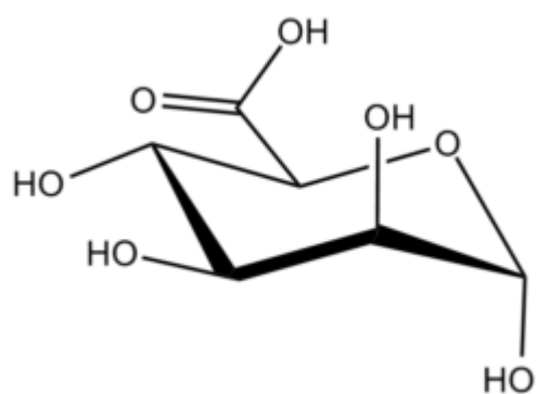
Mannopyranuronic ?-D
