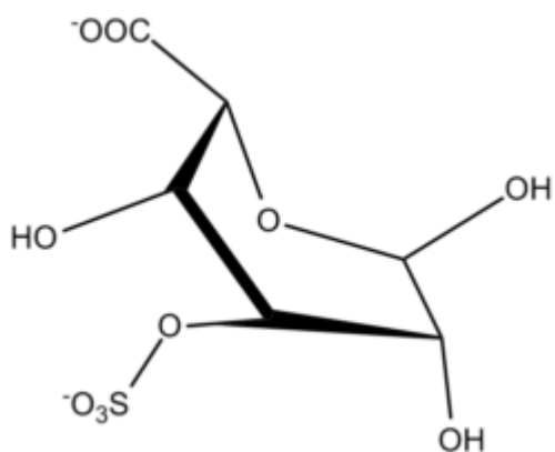
Idopyranuronic 2-S \alpha -L (2S0 conf.)
