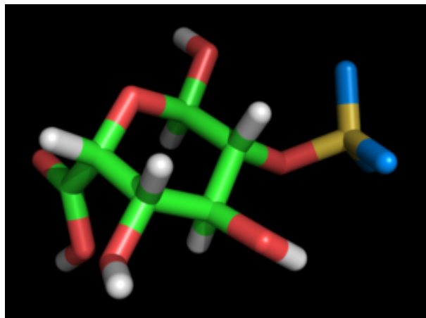
Idopyranuronic ?-L (1C4 conf.)
