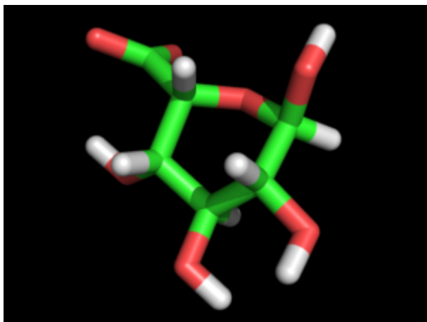
Idopyranuronic ?-L (2S0 Conf.)
