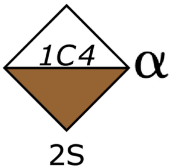
Idopyranuronic ?-L (1C4 conf.)
