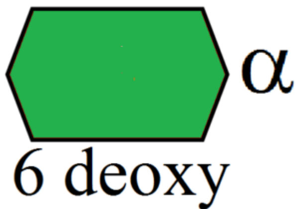
Heptose 6 deoxy
