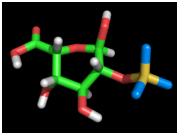
Idopyranuronic 2-S \alpha -L (2S0 conf.)
