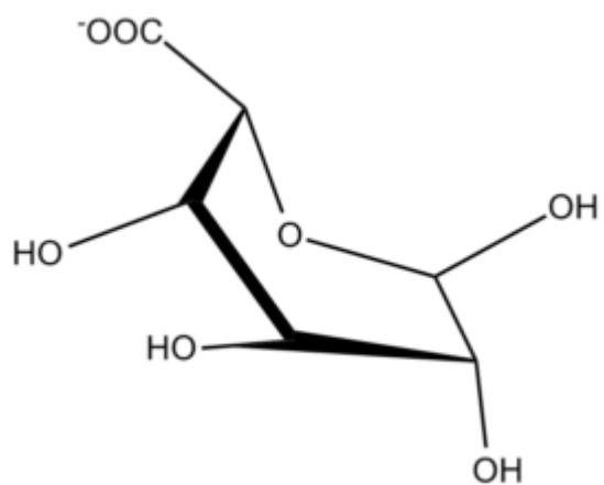
Idopyranuronic ?-L (2S0 Conf.)
