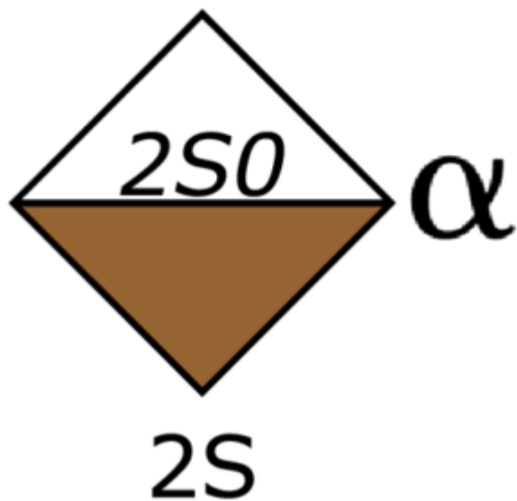
Idopyranuronic 2-S \alpha -L (2S0 conf.)
