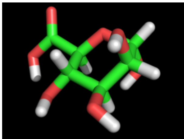
Mannopyranuronic ?-D
