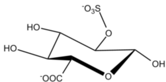
Idopyranuronic ?-L (1C4 conf.)
