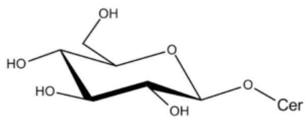
Gluco pyranose ?-D 1-1 Cer
