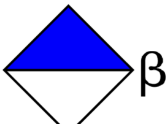
Glucopyranuronic 6-S Î²-D
