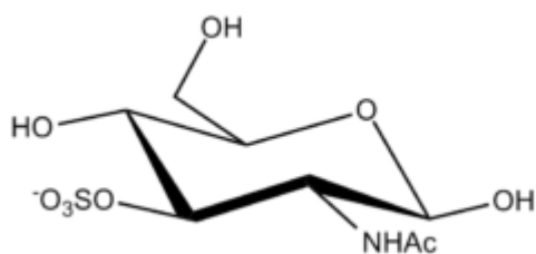
N-Acetyl Glucosamine 3-S ?-D
