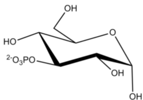
Glucopyranose 3-P Î±-D
