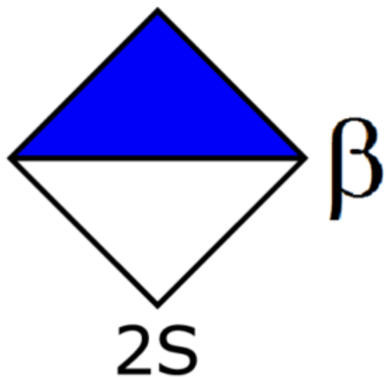
Glucopyranuronic 2-S ?-D
