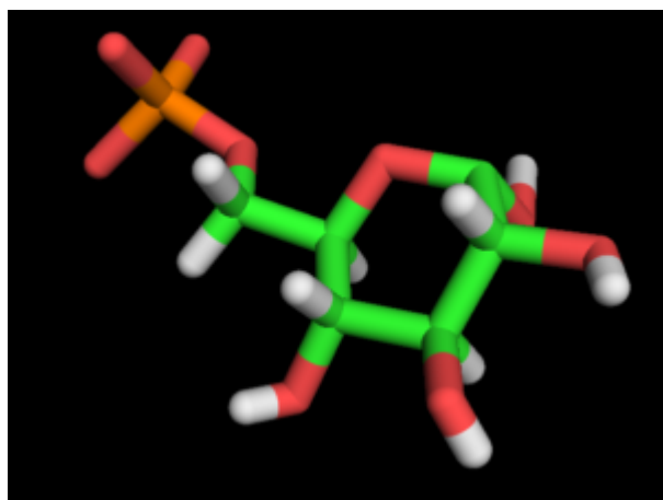
Glucopyranose 6-P ?-D
