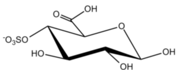
Glucopyranuronic 4-S Î²-D
