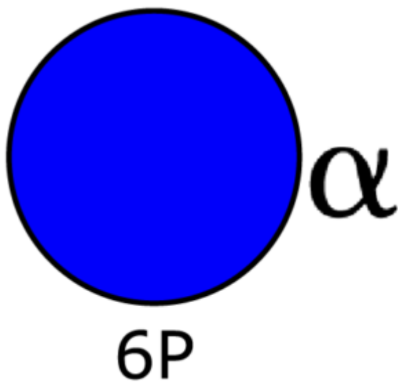
Glucopyranose 6-P ?-D
