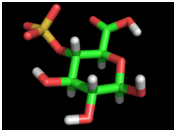
Glucopyranuronic 4-S Î²-D
