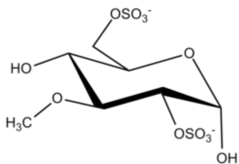
Glucopyranose 2-S,3-OMe,6-S Î±-D
