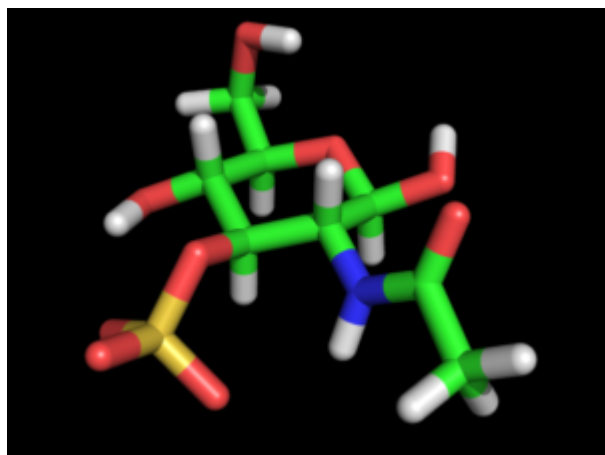
N-Acetyl Glucosamine 3-S ?-D
