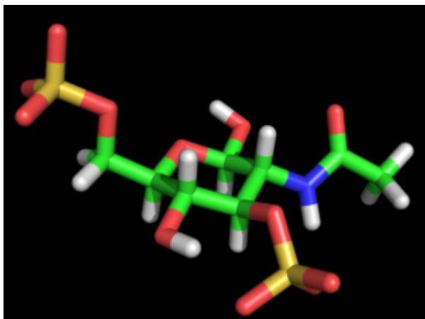
N-Acetyl Glucosamine 3,6-S ?-D
