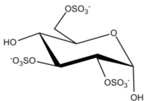
Glucopyranose 2,3,6-S ?-D
