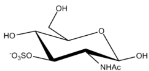
N-Acetyl Glucosamine 3-S \beta -D
