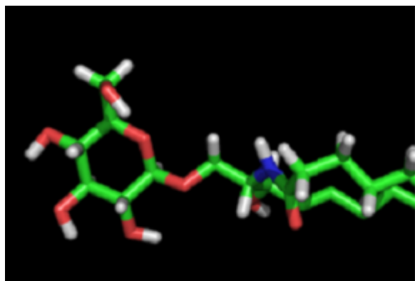
Gluco pyranose ?-D 1-1 Cer
