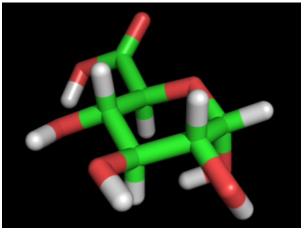
Glucopyranuronic ?-D
