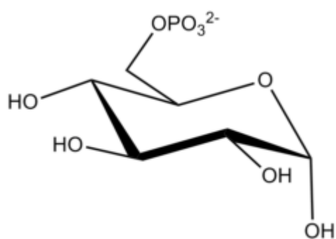
Glucopyranose 6-P Î±-D
