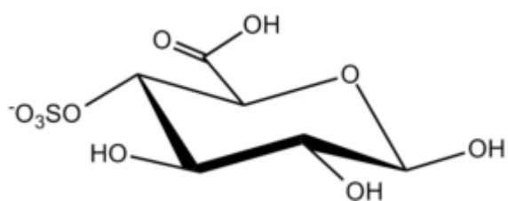
Glucopyranuronic 4-S ?-D
