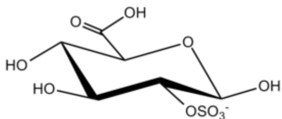
Glucopyranuronic 2-S ?-D
