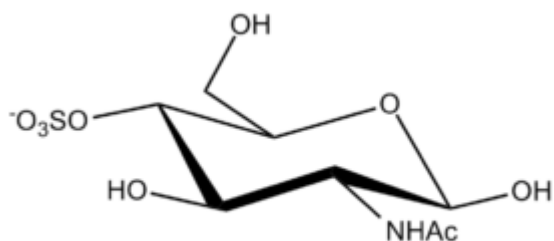
N-Acetyl Glucosamine 4-S ?-D
