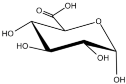
Glucopyranuronic ?-D
