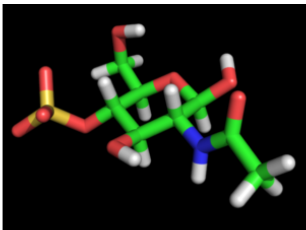
N-Acetyl Glucosamine 4-S ?-D
