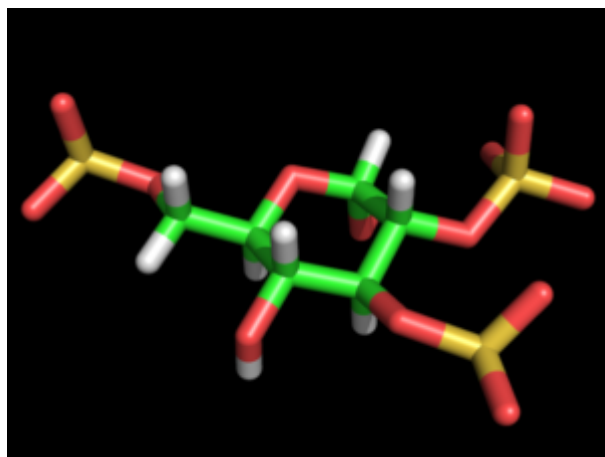
Glucopyranose 2,3,6-S ?-D
