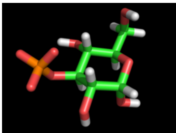
Glucopyranose 3-P ?-D
