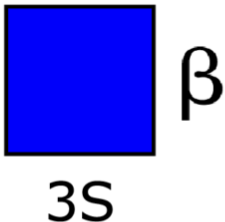
N-Acetyl Glucosamine 3-S ?-D
