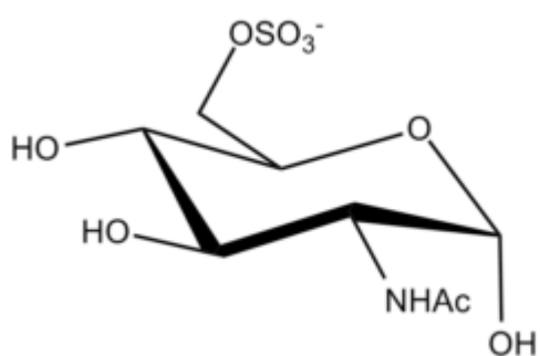
N-Acetyl Glucosamine 6-S ?-D
