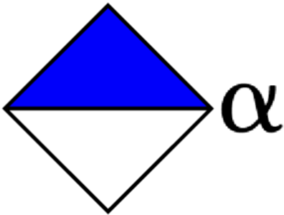
Glucopyranuronic ?-D
