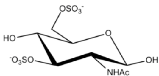
N-Acetyl Glucosamine 3,6-S ?-D
