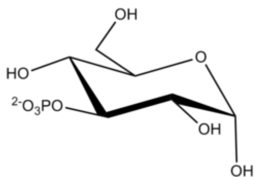
Glucopyranose 3-P ?-D
