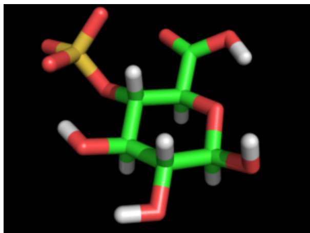
Glucopyranuronic 4-S ?-D
