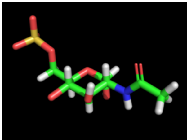
N-Acetyl Glucosamine 6-S ?-D
