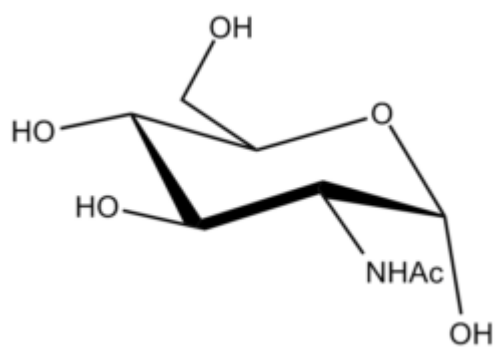
N-Acetyl Glucosamine \hat{1}\pm -D
