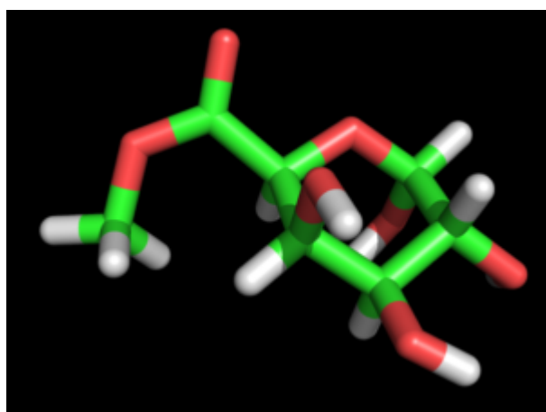
Galactopyranuronic 6OMe ?-D
