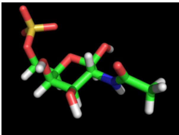
N-Acetyl Galactosamine 6-Sulfate ?-D
