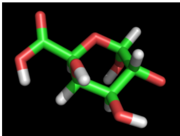
Galactopyranuronic ?-D
