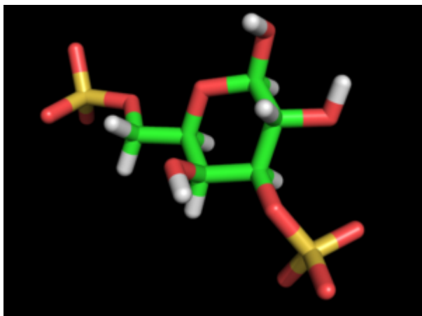
Galactopyranose 3,6-Sulfate ?-D
