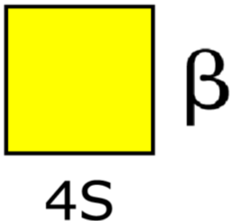
N-Acetyl Galactosamine 4-Sulfate ?-D
