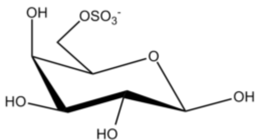
Galactopyranose 6-Sulfate ?-D
