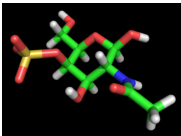
N-Acetyl Galactosamine 4-Sulfate ?-D
