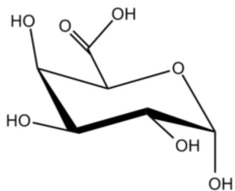
Galactopyranuronic ?-D
