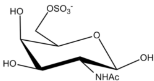
N-Acetyl Galactosamine 6-Sulfate ?-D
