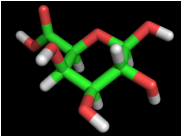
Galactopyranuronic ?-D
