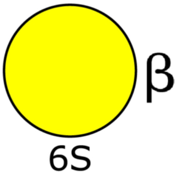
Galactopyranose 6-Sulfate ?-D
