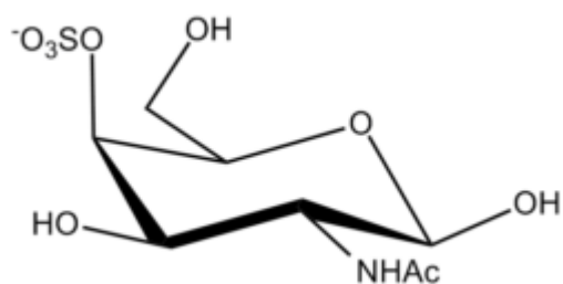
N-Acetyl Galactosamine 4-Sulfate ?-D
