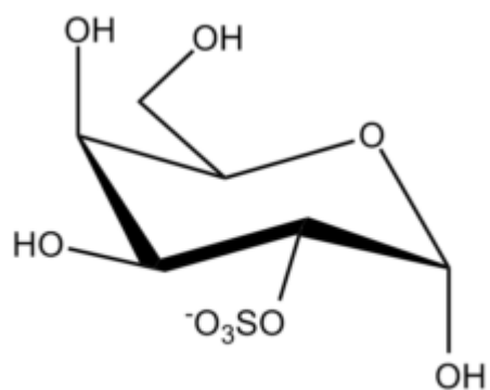
Galactopyranose 2-Sulfate ?-D
