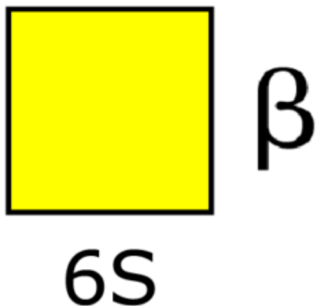
N-Acetyl Galactosamine 6-Sulfate ?-D
