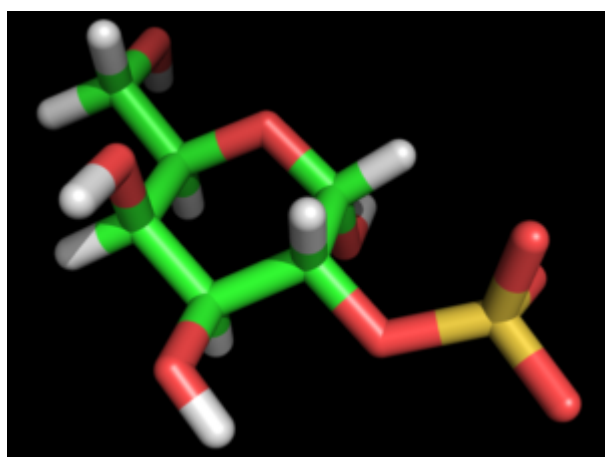
Galactopyranose 2-Sulfate ?-D
