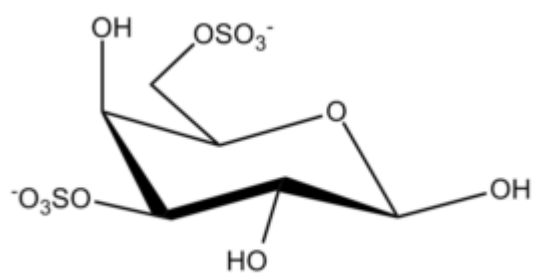
Galactopyranose 3,6-Sulfate ?-D
