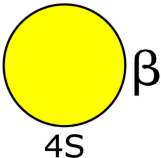
32a. Galactopyranose 4-Sulfate \hat{1}^2 -D
