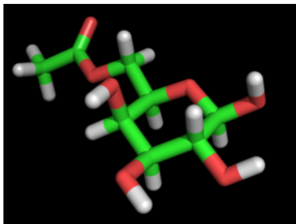
Galactopyranose 6-OAc ?-D
