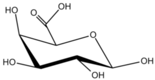
Galactopyranuronic ?-D
