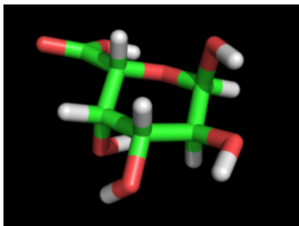
Galactopyranuronic ?-L
