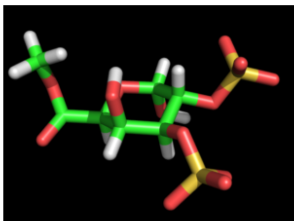
Galactopyranuronic 2,3-Sulfate 6OMe ?-D
