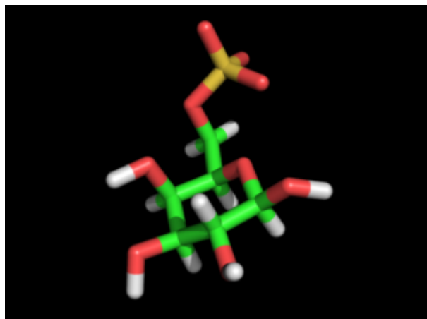
Galactopyranose 6-Sulfate ?-D
