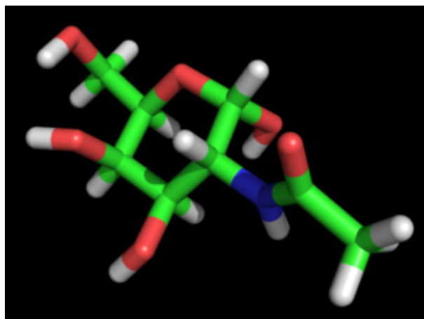
N-Acetyl Galactosamine ?-D
