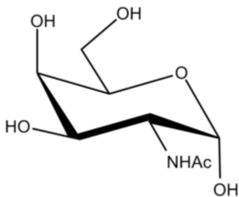
N-Acetyl Galactosamine ?-D
