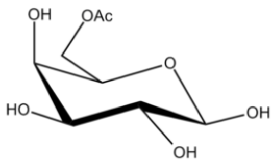
Galactopyranose 6-OAc ?-D
