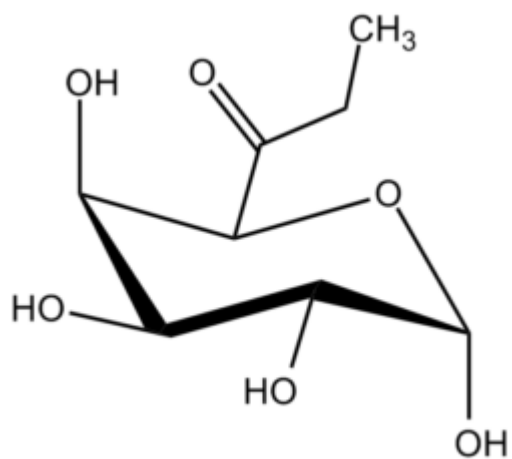
Galactopyranuronic 6OMe ?-D
