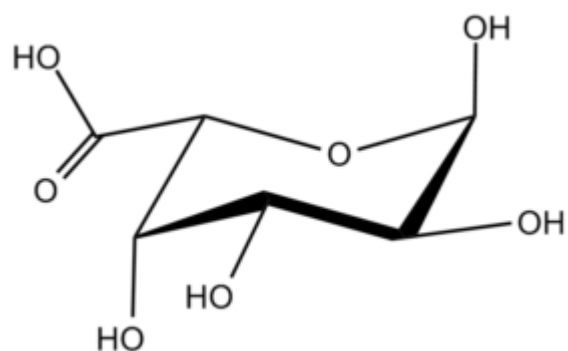
Galactopyranuronic ?-L
