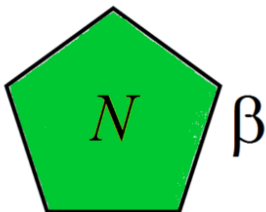
Fructofuranose \beta -D Northern Conformation
