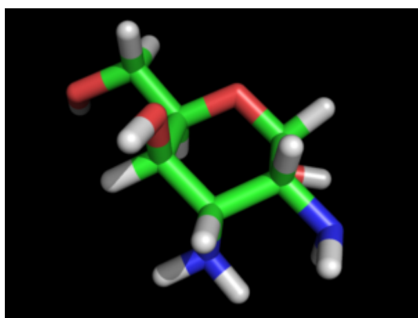
Glucose
