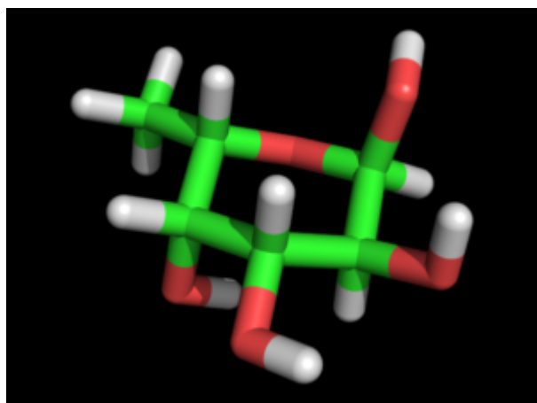
Fucopyranose ?-L
