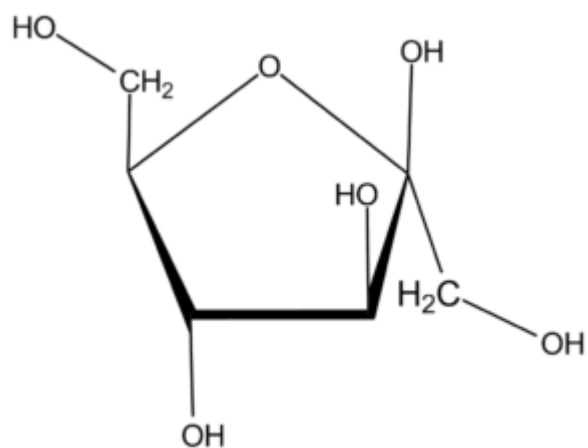
Fructofuranose \beta -D Northern Conformation
