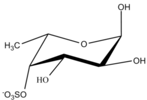
Fucopyranose 4-Sulfate ?-L
