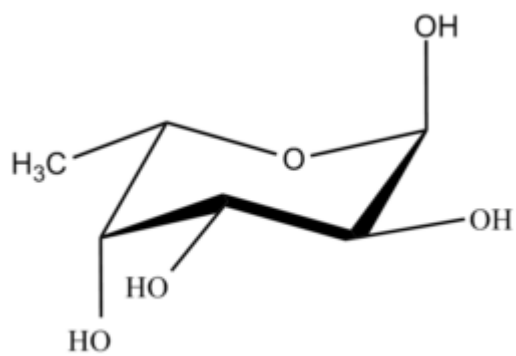
Fucopyranose ?-L
