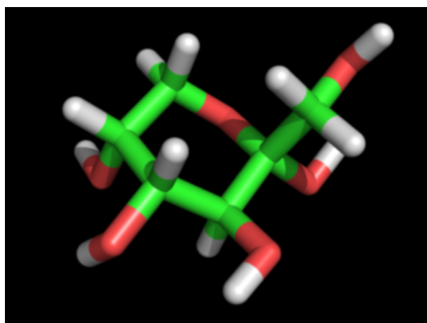
?-D-Fructopyranose
