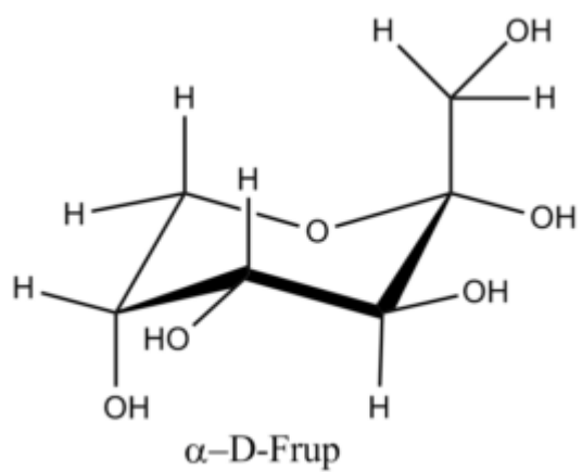
?-D-Fructopyranose
