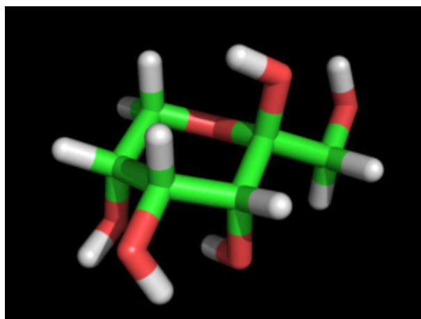
?-D-Psicopyranose
