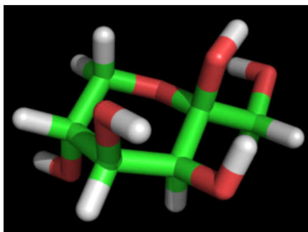
?-D-Tagatopyranose
