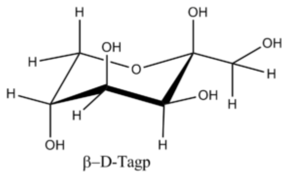
?-D-Tagatopyranose
