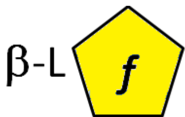
?-L-Tagatofuranose
