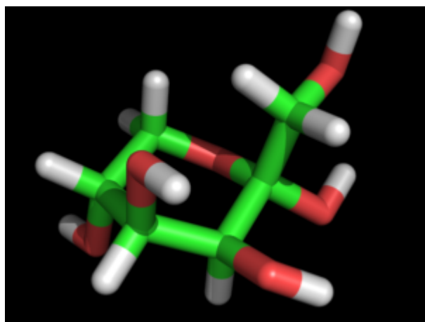
?-D-Tagatopyranose
