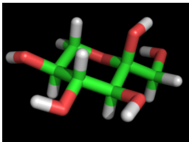
?-L-Sorbopyranose
