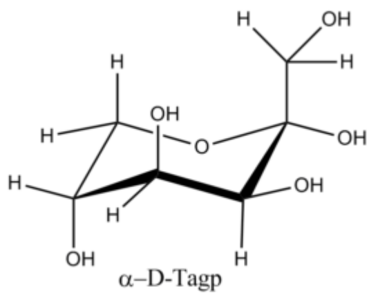
?-D-Tagatopyranose
