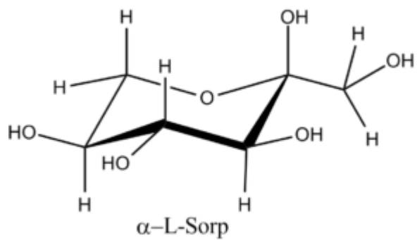
?-L-Sorbopyranose
