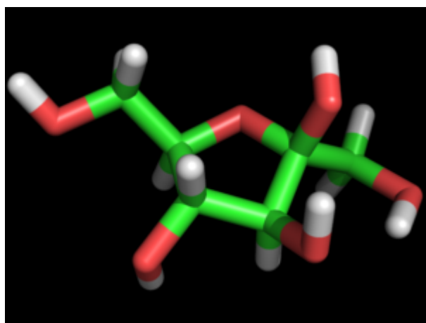
?-D-Fructofuranose
