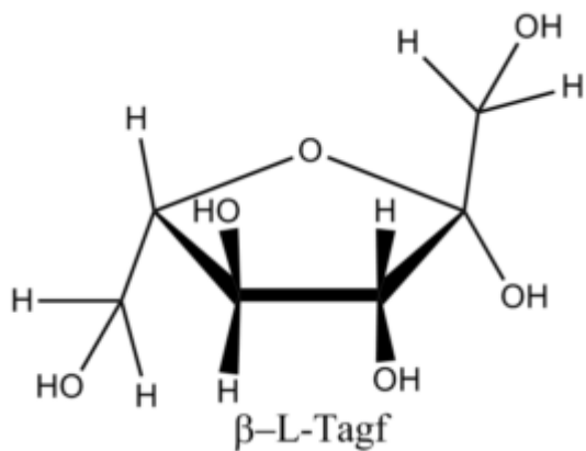
?-L-Tagatofuranose
