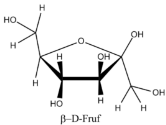
?-D-Fructofuranose
