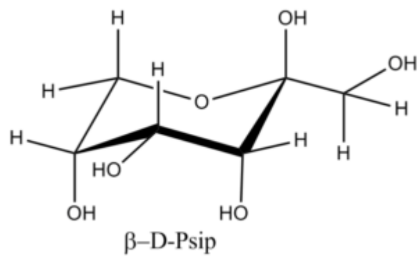
?-D-Psicopyranose
