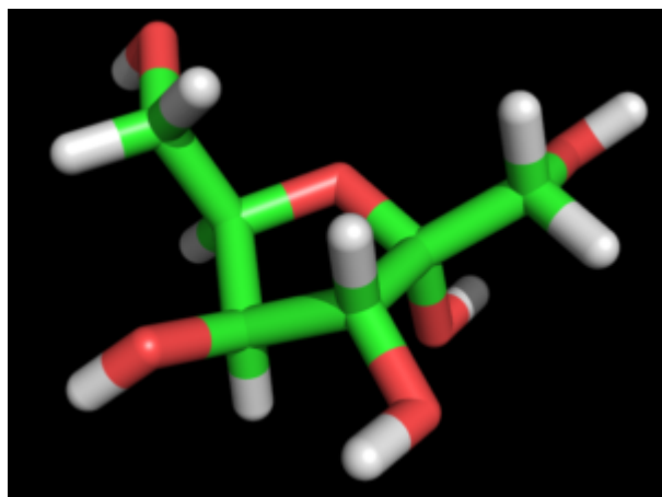
?-D-Sorbofuranose
