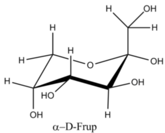
?-D-Fructopyranose
