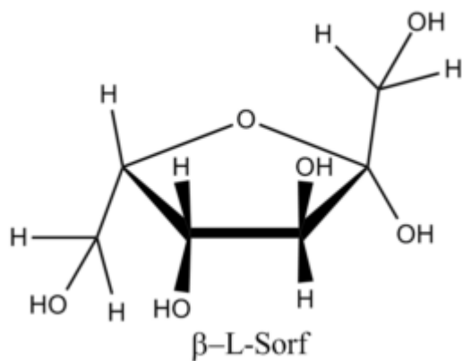
?-L-Sorbofuranose
