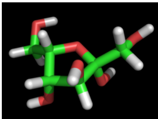
?-L-Sorbofuranose
