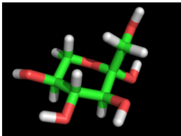
1S02
