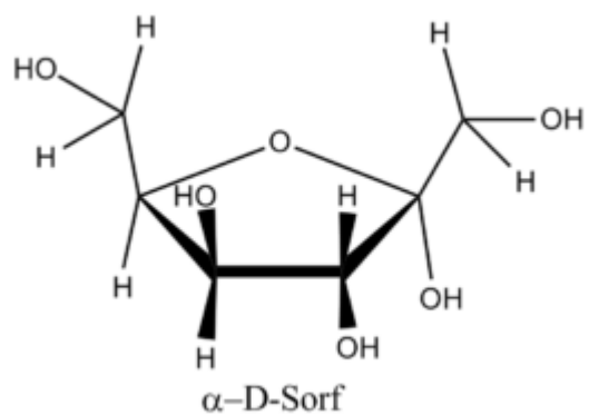
?-D-Sorbofuranose
