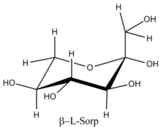
?-L-Sorbopyranose
