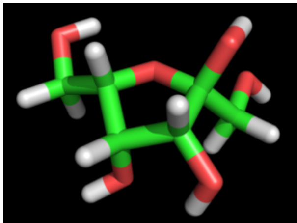
?-L-Tagatofuranose
