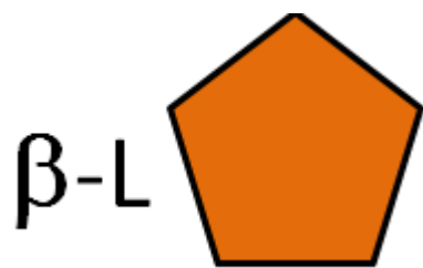
?-L-Sorbopyranose
