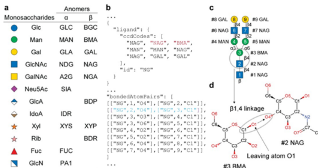
Figure. Glycans specification using Chemical Component Dictionary (CCD) and bondedAtomPairs (BAP) syntax in AlphaFold 3. a , Representative CCD codes for common human monosaccharides. b , Partial JSON script used to generate G2 N-linked glycan. c , SNFG representation of G2 N-linked glycan with residue numbering equivalent to what is used in the JSON modeling input file. The order of the monosaccharides in the JSON file ccdCodes list corresponds with the residue numbering in the SNFG representation. d , Demonstration of a \beta 1,4 linkage between GlcNAc and Man, specified by the second and third CCD entries (red NAG and BMA) in panel b . The glycosidic bond is defined by the bondedAtomPairs (BAP) field (blue in panel b ), specifying a bond between the O4 atom of NAG and the C1 atom of BMA (gray oval in panel d ). The entry in the bondedAtomPairs (BAP) list leads to covalent bond formation between the respective hydroxyl oxygen (O4 of NAG) and the anomeric C1 (C1 of BMA) with the removal of the \hat{\imath}^2 -linked O1 (leaving atom) on the C1 of BMA. The resulting glycosidic linkage retains the anomeric configuration at C1 of the original CCD entry ( \hat{\imath}^2 -linkage for BMA).
