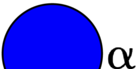
Glucopyranose 2-S,3-OMe,6-S \hat{\pm} -D
