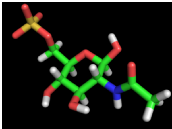
N-Acetyl Glucosamine 6-S \beta -D
