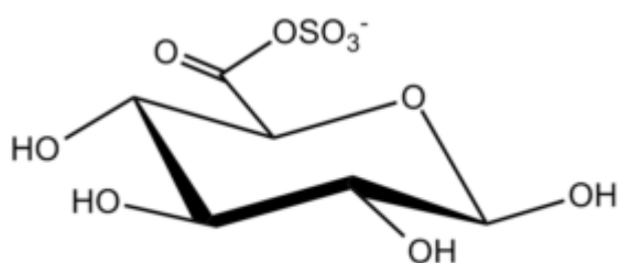
Glucopyranuronic 6-S Î²-D
