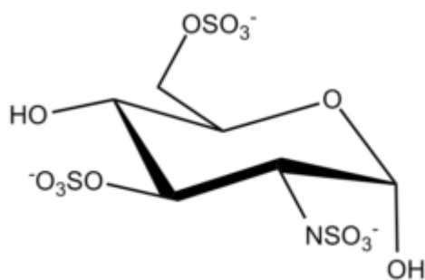
Glucosamine NS 3,6-S \hat{\pm} -D
