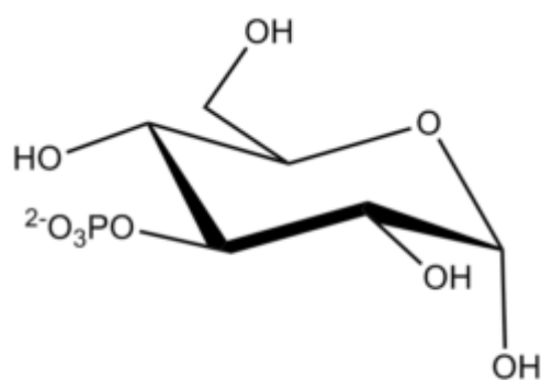
Glucopyranose 3-P \hat{1}\pm -D
