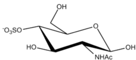
N-Acetyl Glucosamine 4-S \beta -D
