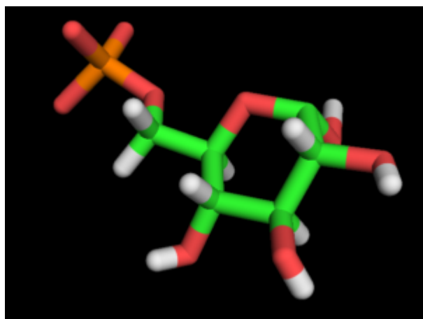
Glucopyranose 6-P \hat{\pm} -D
