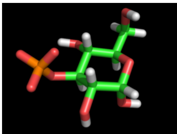
Glucopyranose 3-P \hat{1}\pm -D
