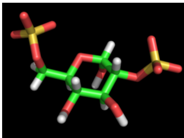
Glucopyranose 2,6-S \hat{\pm} -D
