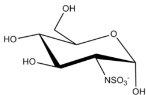
Glucosamine NS \hat{\pm} -D
