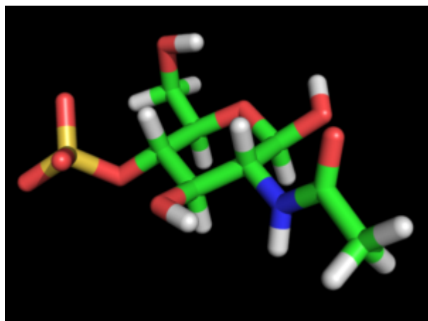
N-Acetyl Glucosamine 4-S \beta -D
