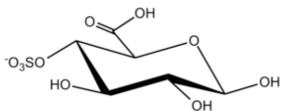
Glucopyranuronic 4-S \beta -D
