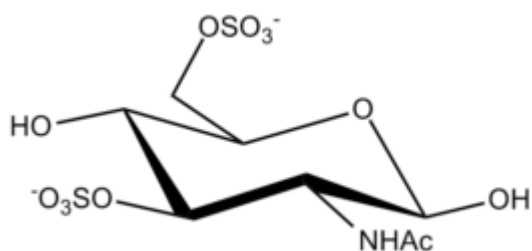
N-Acetyl Glucosamine 3,6-S \beta -D
