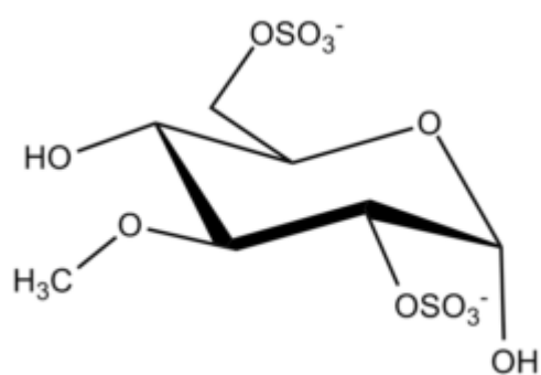
Glucopyranose 2-S,3-OMe,6-S \hat{I}\pm -D
