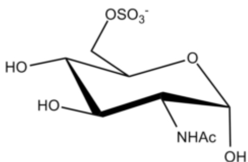
N-Acetyl Glucosamine 6-S \beta -D
