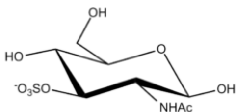
N-Acetyl Glucosamine 3-S \beta -D
