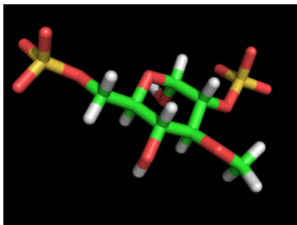
Glucopyranose 2-S,3-OMe,6-S \hat{I}\pm -D
