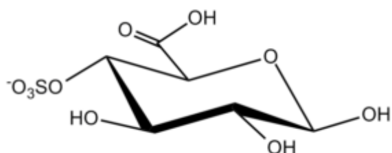
Glucopyranuronic 4-S \beta -D
