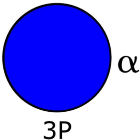
Glucopyranose 3-P \hat{\pm} -D
