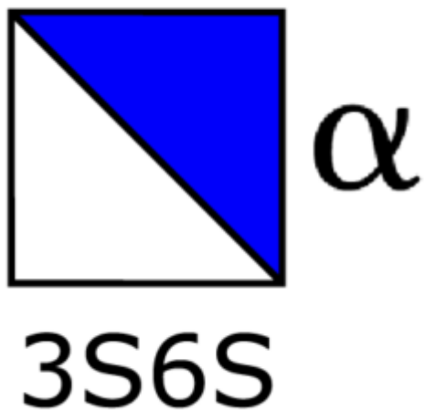
Glucosamine NS 3,6-S \hat{\pm} -D
