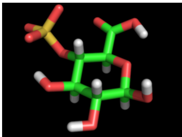
Glucopyranuronic 4-S \beta -D
