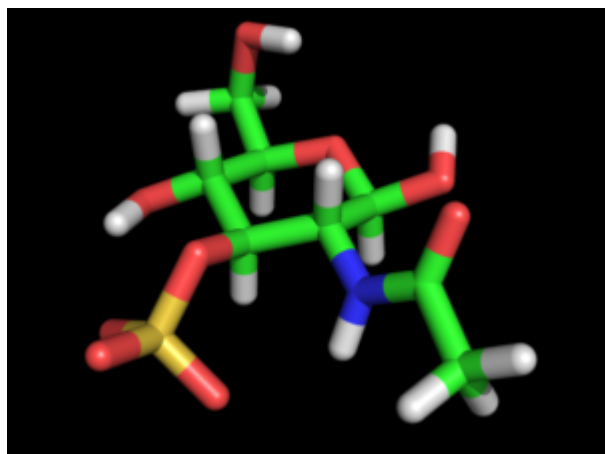
N-Acetyl Glucosamine 3-S \beta -D
