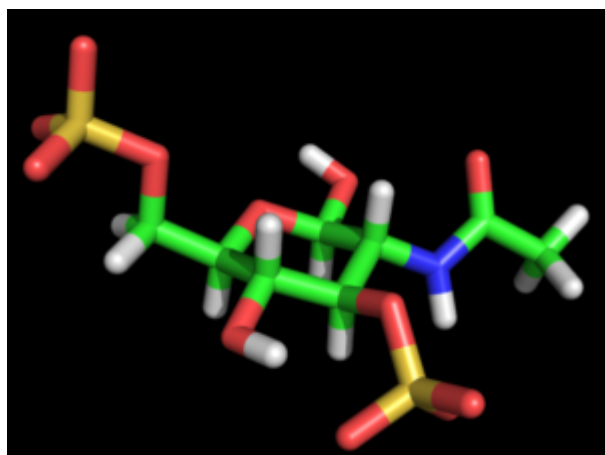
N-Acetyl Glucosamine 3,6-S \beta -D
