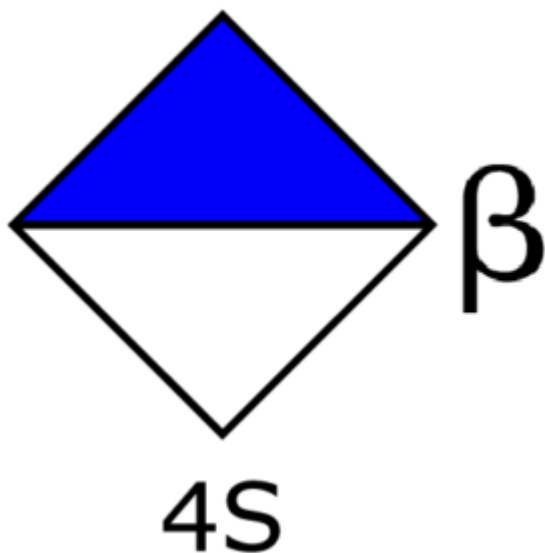
Glucopyranuronic 4-S \beta -D
