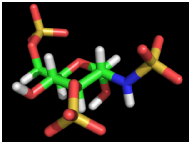
Glucosamine NS 3,6-S \hat{\pm} -D
