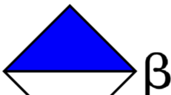
Glucopyranuronic 4-S \hat{1}^2 -D
