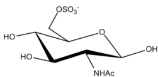
N-Acetyl Glucosamine 6-S \beta -D
