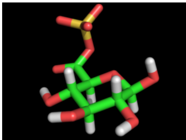
Glucopyranuronic 6-S Î²-D
