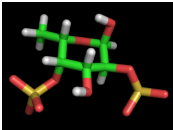
Fucopyranose 2, 4-Sulfate \hat{\pm} -L
