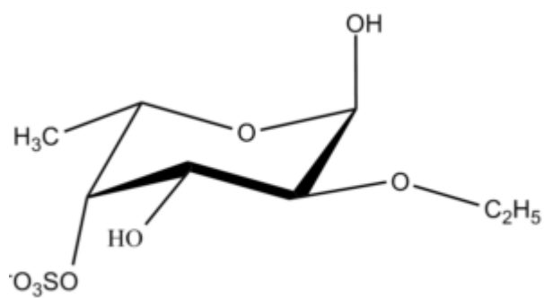
Fucopyranose 2-Ethyl 4-Sulfate \hat{\pm} -L
