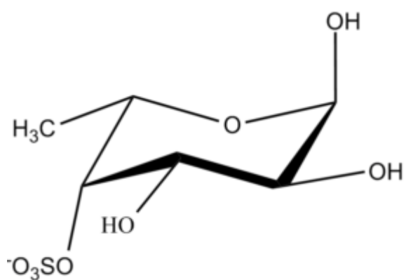
Fucopyranose 4-Sulfate \hat{\pm} -L
