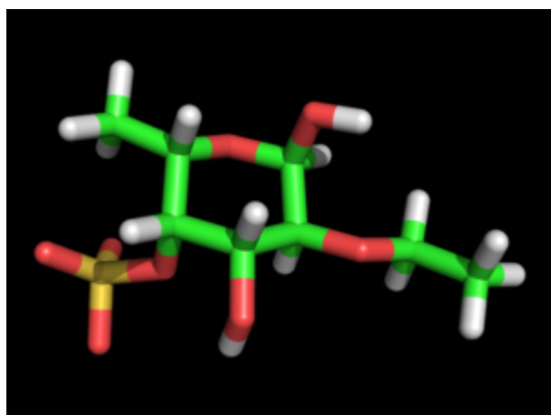
Fucopyranose 2-Ethyl 4-Sulfate \hat{\pm} -L
