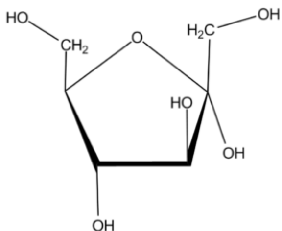
Fructofuranose Î±-D Southern Conformation
