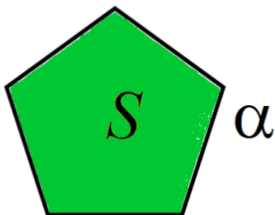
Fructofuranose Î±-D Southern Conformation
