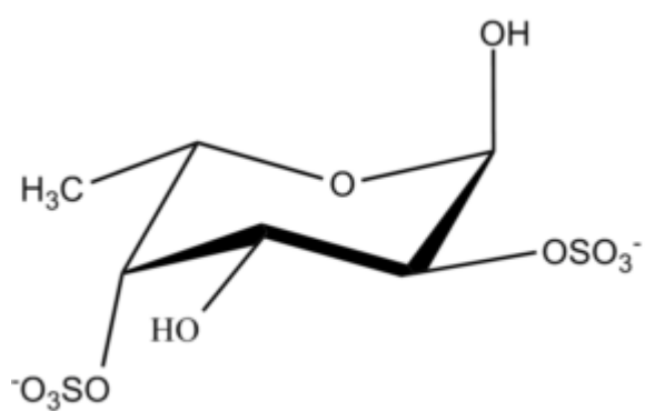
Fucopyranose 2, 4-Sulfate \hat{\pm} -L
