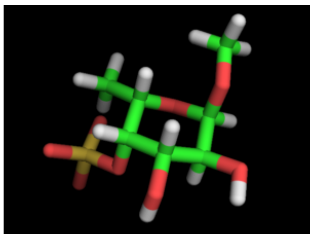
Fucopyranose 4-Sulfate \hat{\pm} -L
