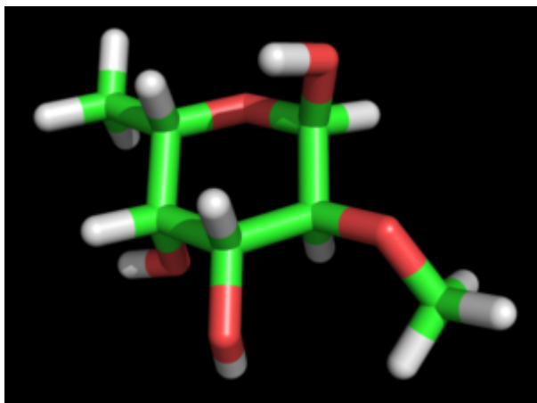
Fucopyranose 2-OMethyl L
