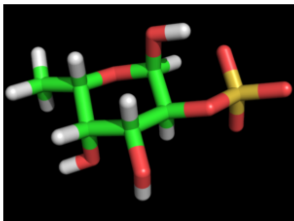
Fucopyranose 2-Sulfate \hat{\pm} -L
