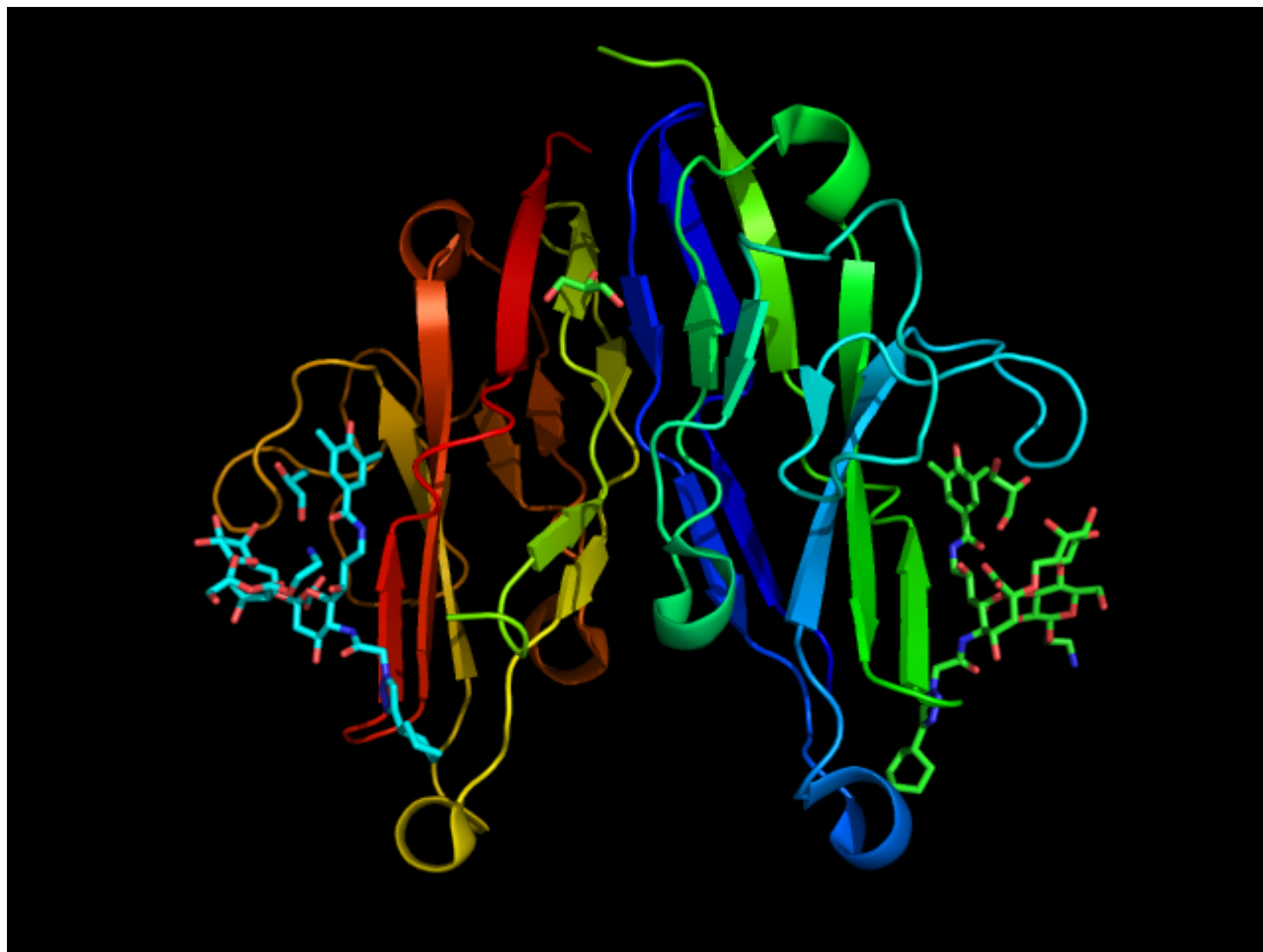
Figure 8. (Top) Crystal structure of CD33 together with ligand 9. PDB code: 6D4A. (Bottom) Main interactions between CD33 and ligand 9. http://www.rcsb.org/3d-view/6d4a
