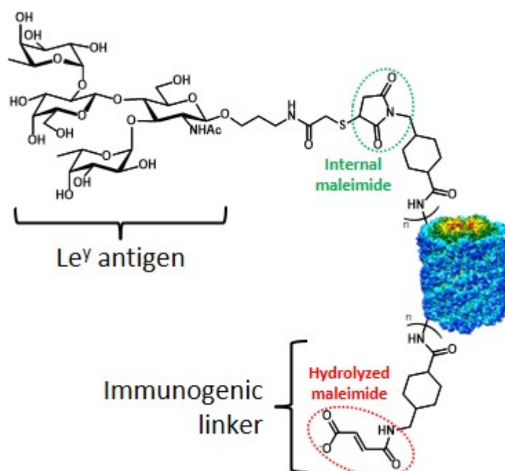
Figure 7. Ley-KLH vaccine conjugate by Boons and co-workers showing the hydrolyzed maleimide function, which caused antigen suppression.
