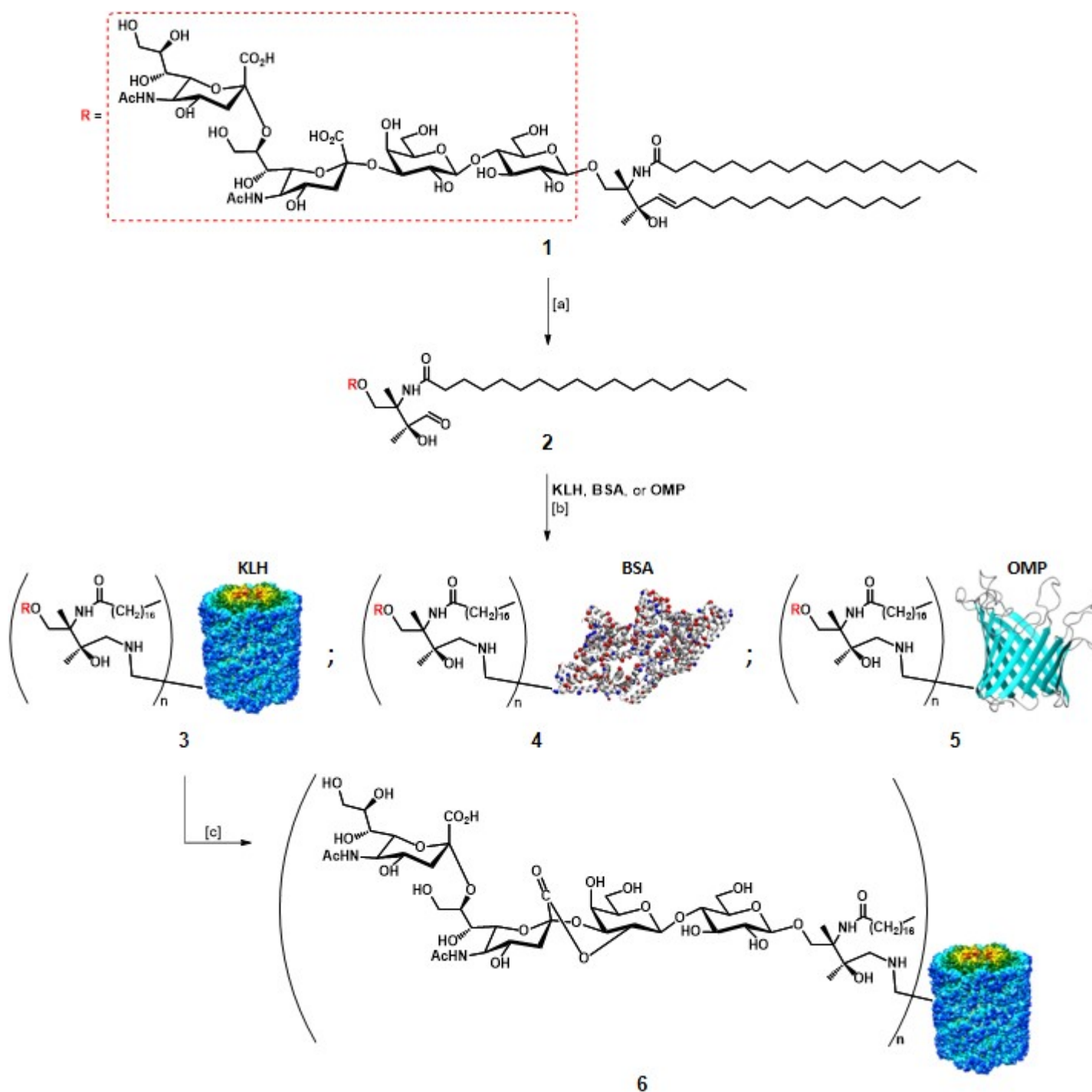
Scheme 1. Synthesis of GD3-protein conjugates. Conditions: [a] \text{O}_3 , MeOH, -78^\circ\text{C} , 30 min., then \text{CH}_3\text{SH} , -78^\circ\text{C} for 30 min., then r.t. for 90 min.; [b] PBS (pH 7.2), \text{NaCNBH}_3 , 37^\circ\text{C} for 48 h.; [c] \text{CH}_3\text{COOH} , 37^\circ\text{C} , 4 h, 80% conversion to lactone form. GD3:protein weight ratio is 0.69, 0.77 and 0.93 for {3}, {4} and {5}, respectively.
