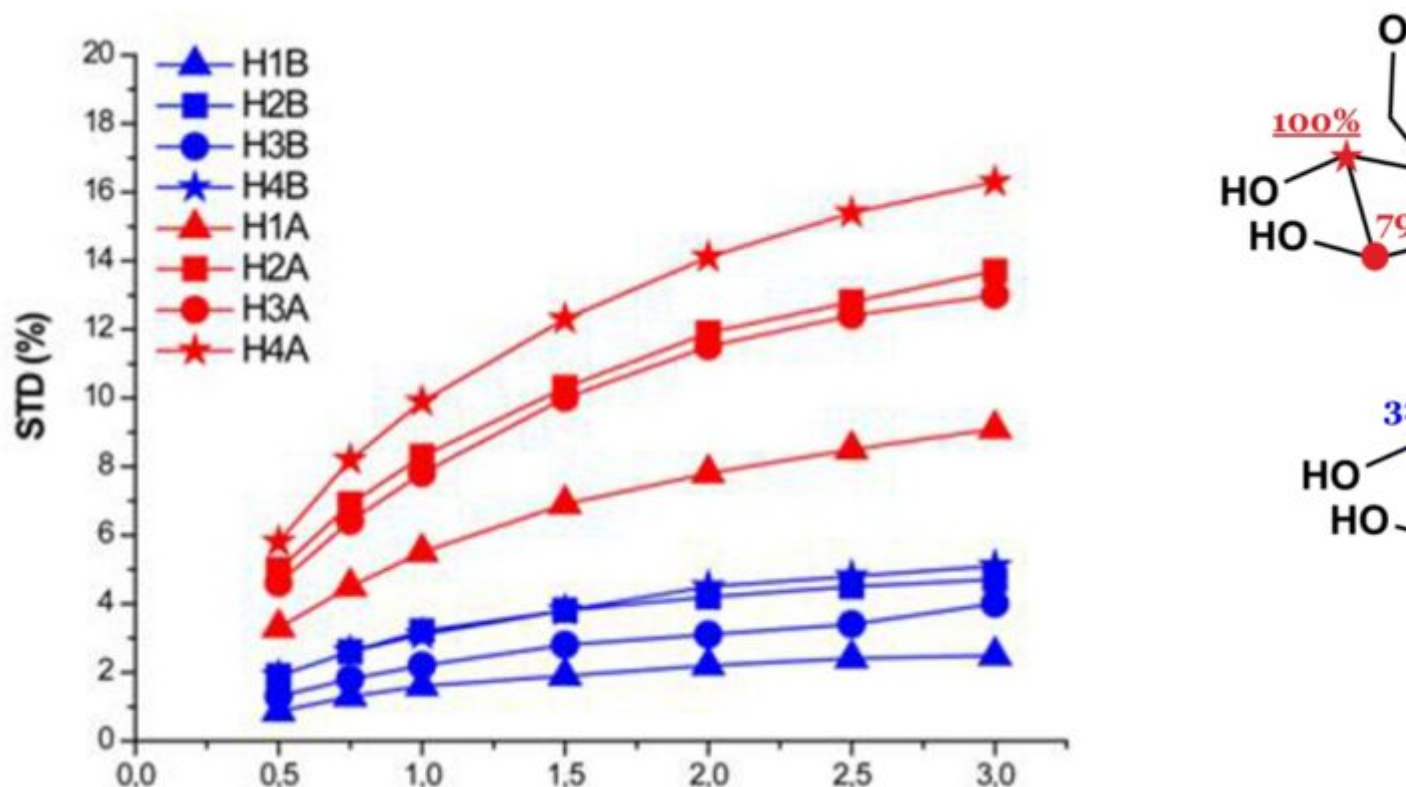
Figure 8. (Left) STD growth curves (absolute values) for the recognition of Man- \hat{1}\pm(1,2) -Man- \hat{1}\pm -O(CH 2 )NH 2 by the anti-HIV-1 human antibody 2G12. (Right) Ligand group epitope mapping, or binding epitope for Man- \hat{1}\pm(1,2) -Man- \hat{1}\pm -O(CH 2 )NH 2 compound. Note that proton H4A receives the highest saturation (thus the 100% is arbitrarily assigned) and is used as reference to calculate the STD percentages of the other protons. Residue of mannose-A makes the main contacts with the protein in the bound state.
