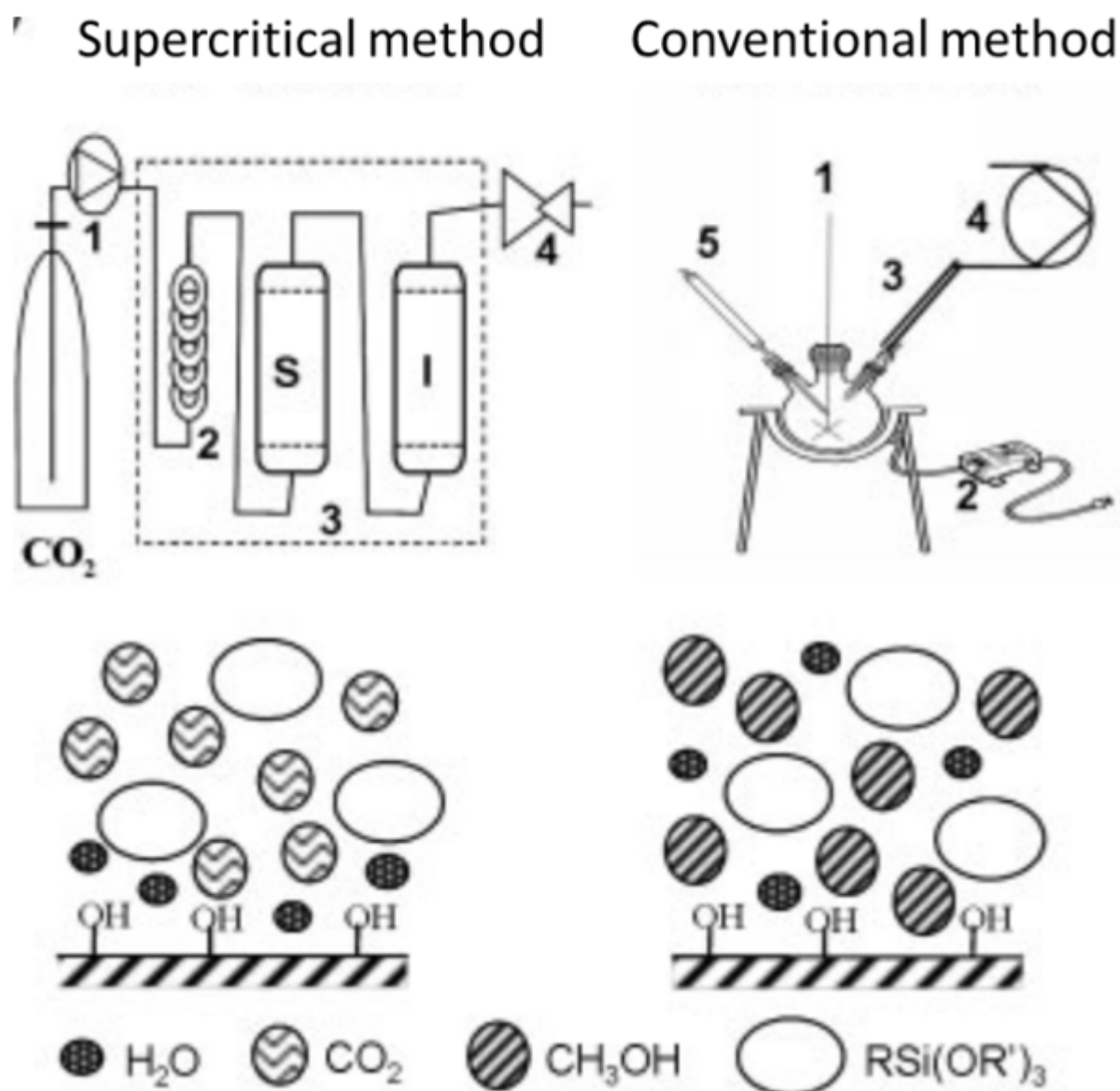
Figure 30: Experimental set-up of silanization in supercritical and conventional conditions and schematic illustration of the reaction (From (Loste et al. 2004)).
