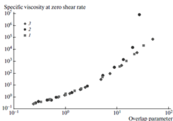
Figure 15. Influence of the overlap parameter on the specific viscosity at zero shear rate and at 25°C: {1} HA in presence of 0.1 M NaCl; {2} chitosan in 0.3 M acetic acid/0.1 M sodium acetate; {3} predicted value from relation established by (Mazeau & Rinaudo, 2012)
