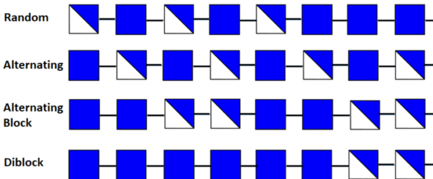
Figure 11. Illustration of theoretical patterns of acetylation (PA) of chitosan polymers, all having the same degree of polymerization and FA = 0.5
