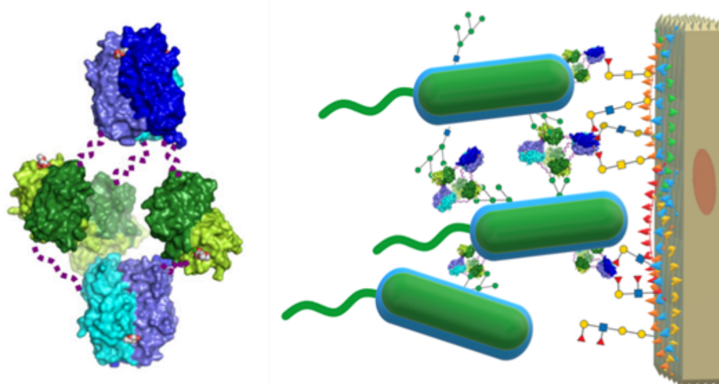
Figure 12. Left: Likely hexameric arrangement of BC2L-C from the SAXS and EM reconstructions. Right: Schematic depiction of the â??cellular bridgeâ?? hypothesis: BC2L-C cross-links B. cenocepacia and human epithelial cells by binding their LPS mannoside and histo-blood fucoside epitopes, respectively. Adapted from Å ulÃ¼k and co-workers (2011).(Sulak et al., 2011)
