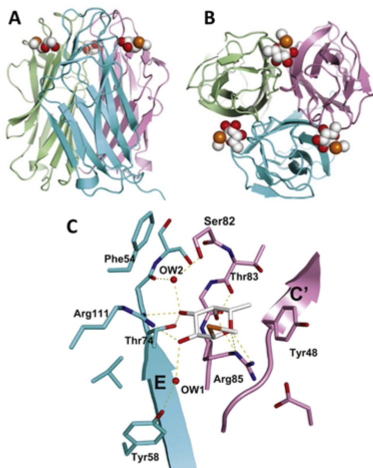
Figure 11. Crystal structure of the N-terminal domain of BC2L-C. A and B: Side view of the homotrimer, ligand is 1- \alpha -Me-Seleno-L-Fucose. C: Details of the binding site of BC2L-C-Nter and interactions with the ligand. Water molecules are depicted as red spheres, ligands as spheres or sticks, H-bonds as yellow dashed lines. Adapted from Å ulÅjk and co-workers (2010). (Sulak et al., 2010)
