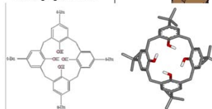
calix[4]arene
