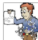
calix[4]arene
