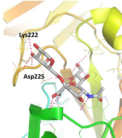
H1 human – 1918
