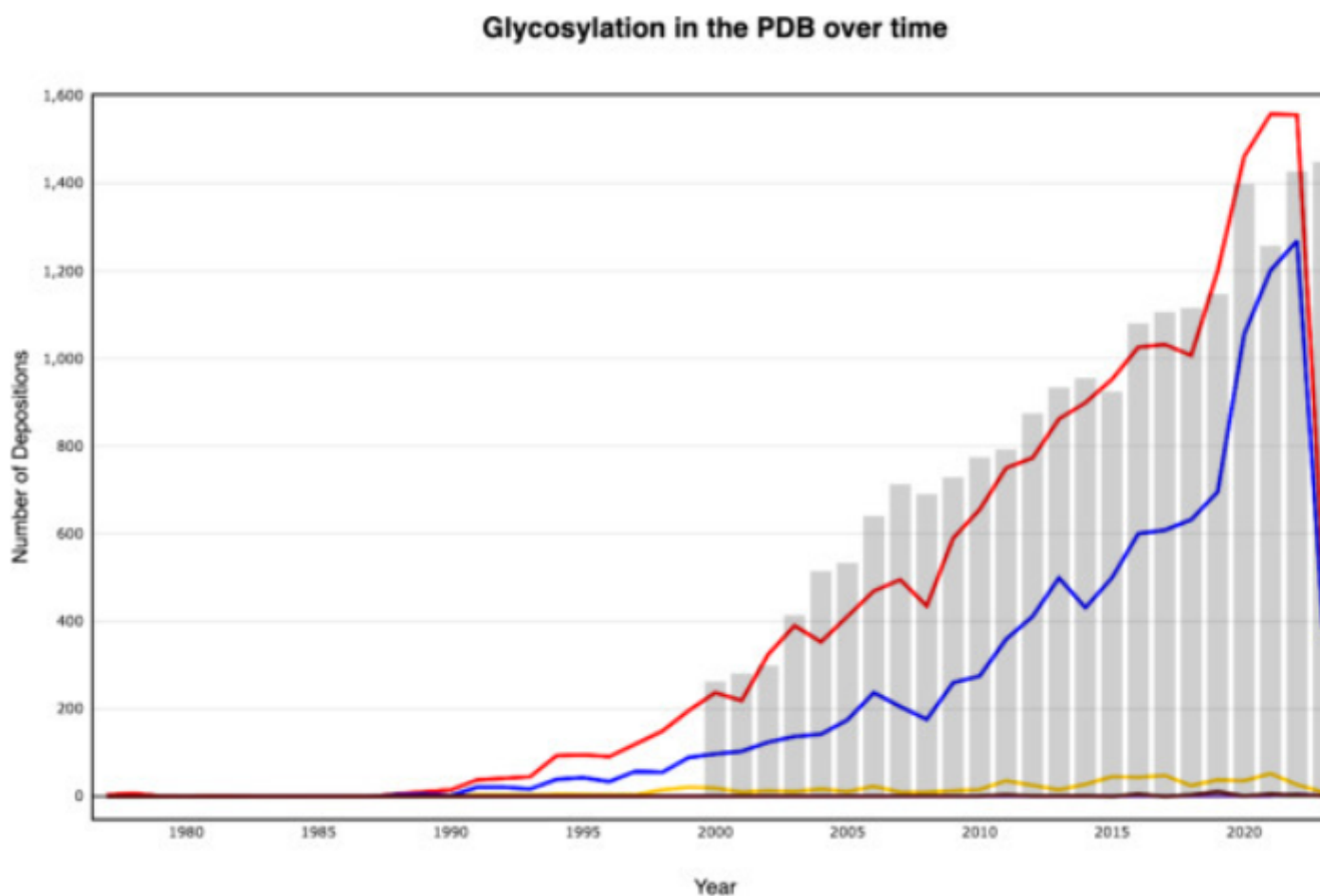
Figure 1: Distribution of carbohydrate-containing structure deposition in the Protein Data Bank over time. Grey bars (right axis) show the total number of structures deposited annually. Lines track structure deposition counts for specific carbohydrate categories (left axis): N -glycans, O -glycans, C -glycans, S -glycans and ligands. The analysis indicates around 10% of yearly deposits are sugar-containing structures. The apparent decline in deposited structures for 2025 likely reflects structures that are still undergoing deposition review or on hold awaiting publication. Data were extracted from the Privateer Database ( Dialpuri, Bagdonas, Schofield, Pham, Holland, and Agirre 2024 )
